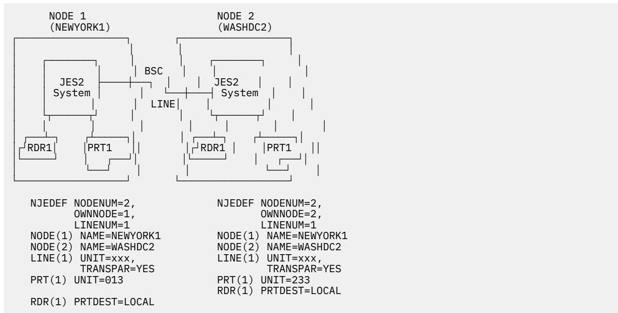
Figure 69: Minimum NJE Configuration (BSC only)
