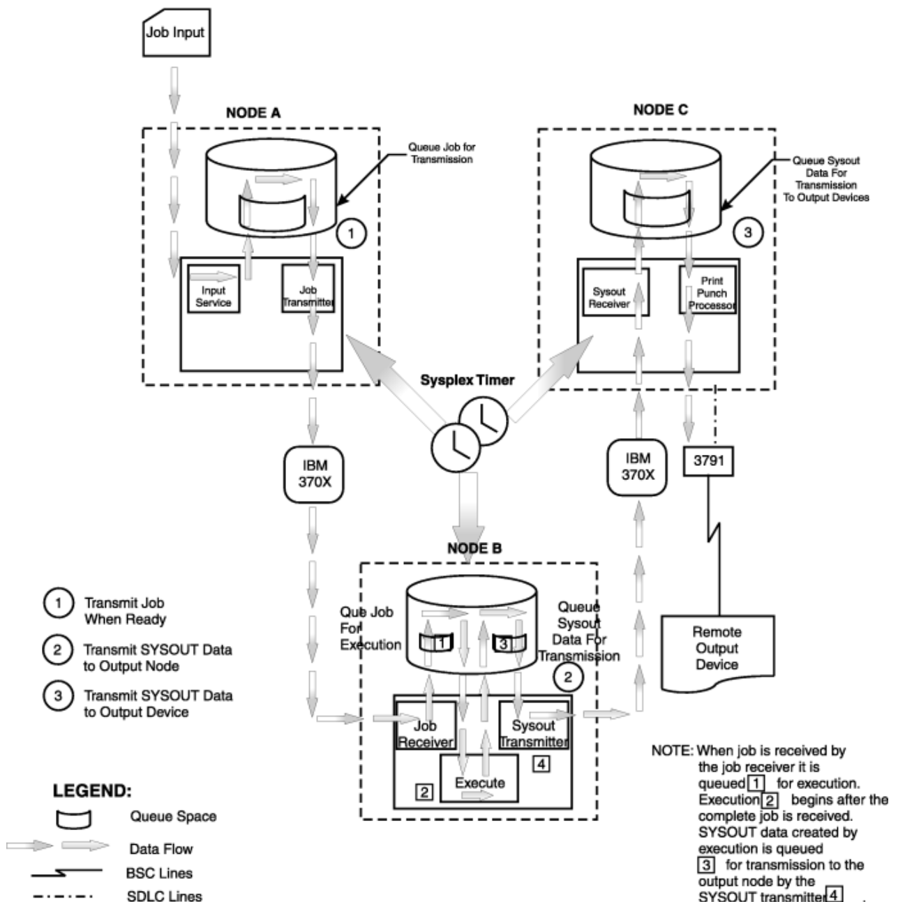
Figure 61: Processing flow through a network
