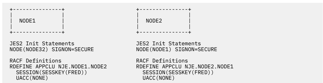
Figure 68: NJE Signon Password Verification for Mixed Levels of JES2
