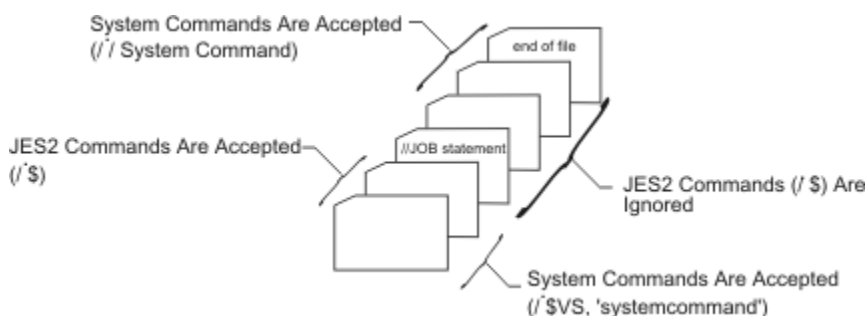
Figure 16: Entering commands from a job stream
