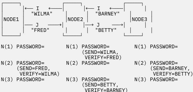
Figure 66: JES2 NJE Signon Password Verification
