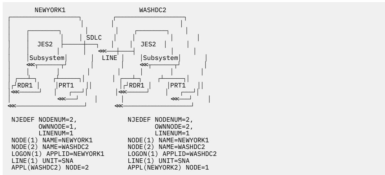
Figure 71: Minimum NJE configuration (SNA)
