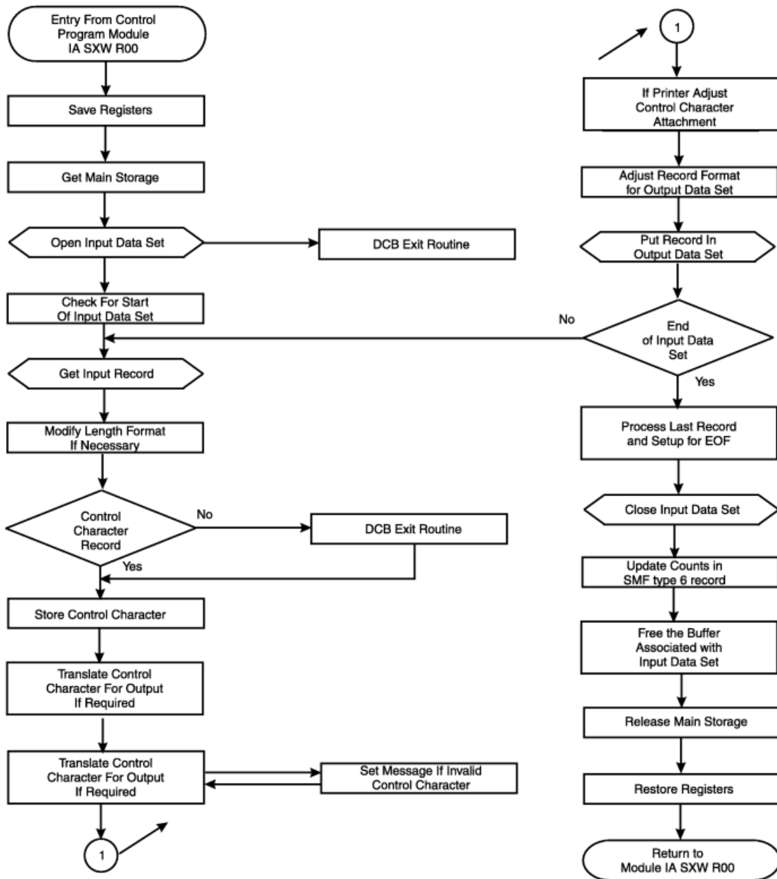
Figure 98: General flow of IBM's output writing routine
