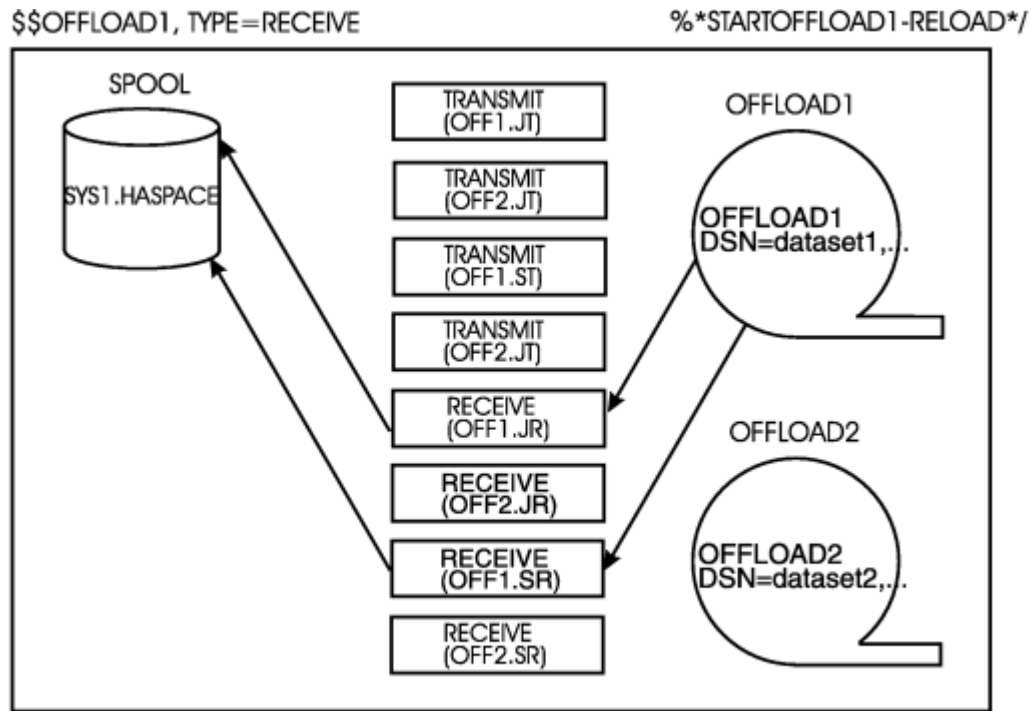
Figure 42: Offload initialization statements and $$ OFFLOADn,TYPE=RECEIVE
